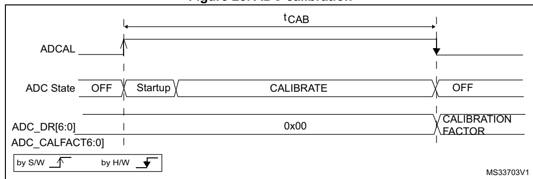
Figure 28. ADC calibration
