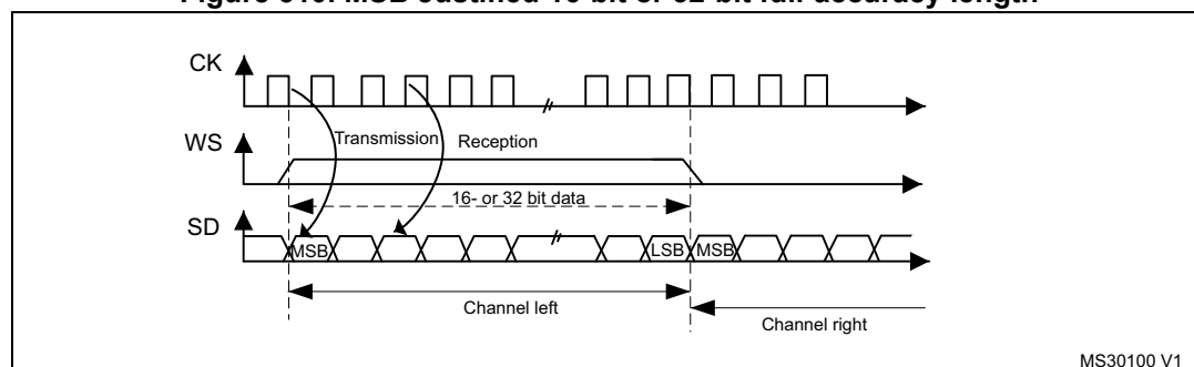
Figure 310. MSB Justified 16-bit or 32-bit full-accuracy length
