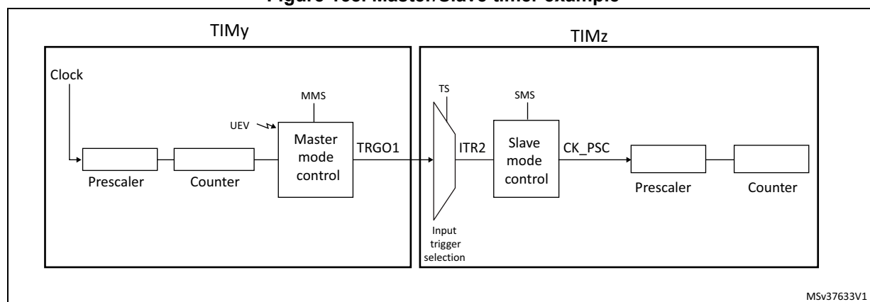
Figure 158. Master/Slave timer example
