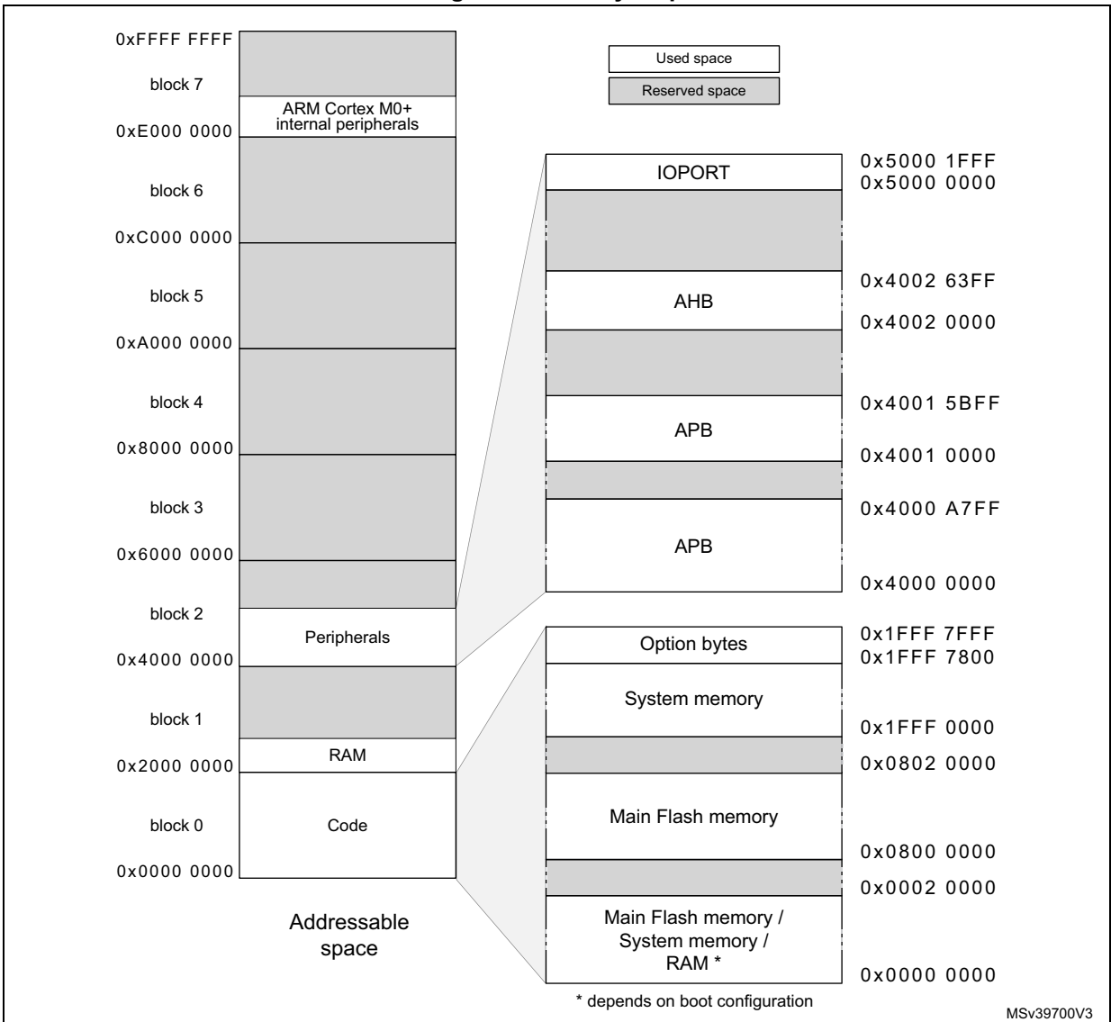
Figure 2. Memory map
