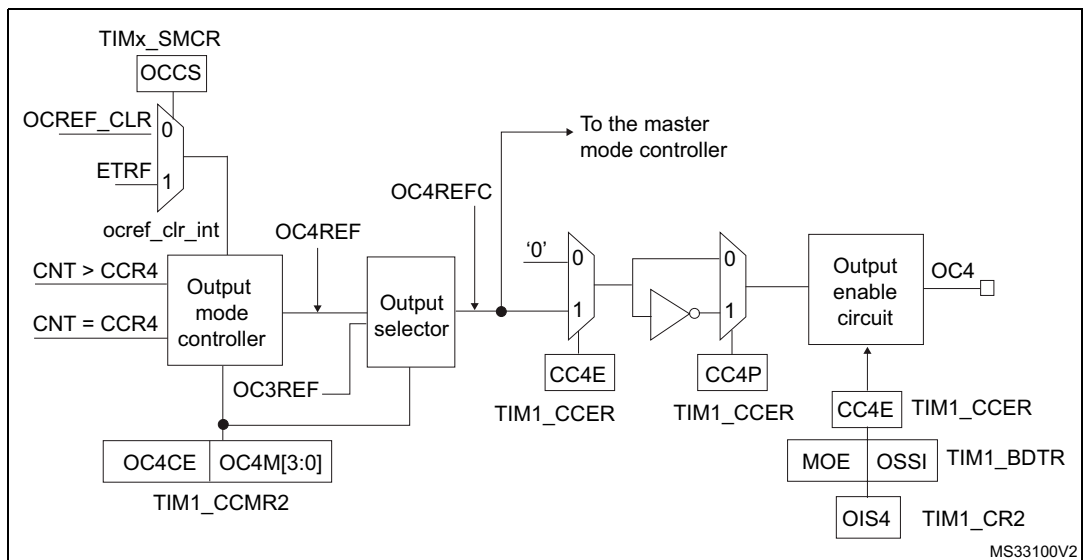
Figure 86. Output stage of capture/compare channel (channel 4)
