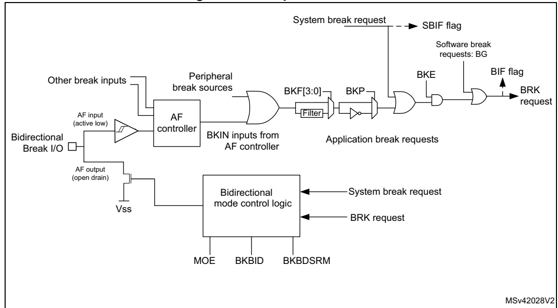
Figure 216. Output redirection
