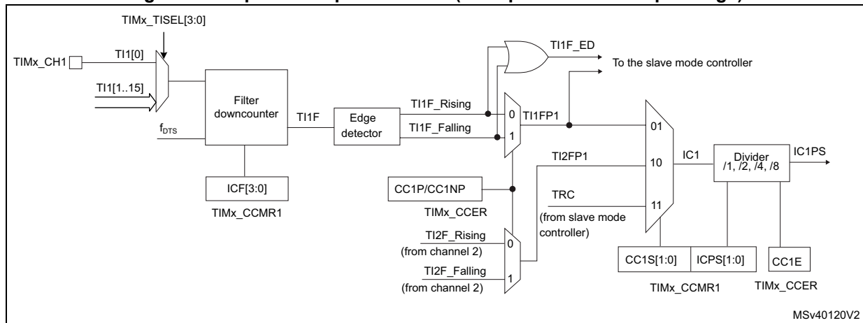
Figure 83. Capture/compare channel (example: channel 1 input stage)
