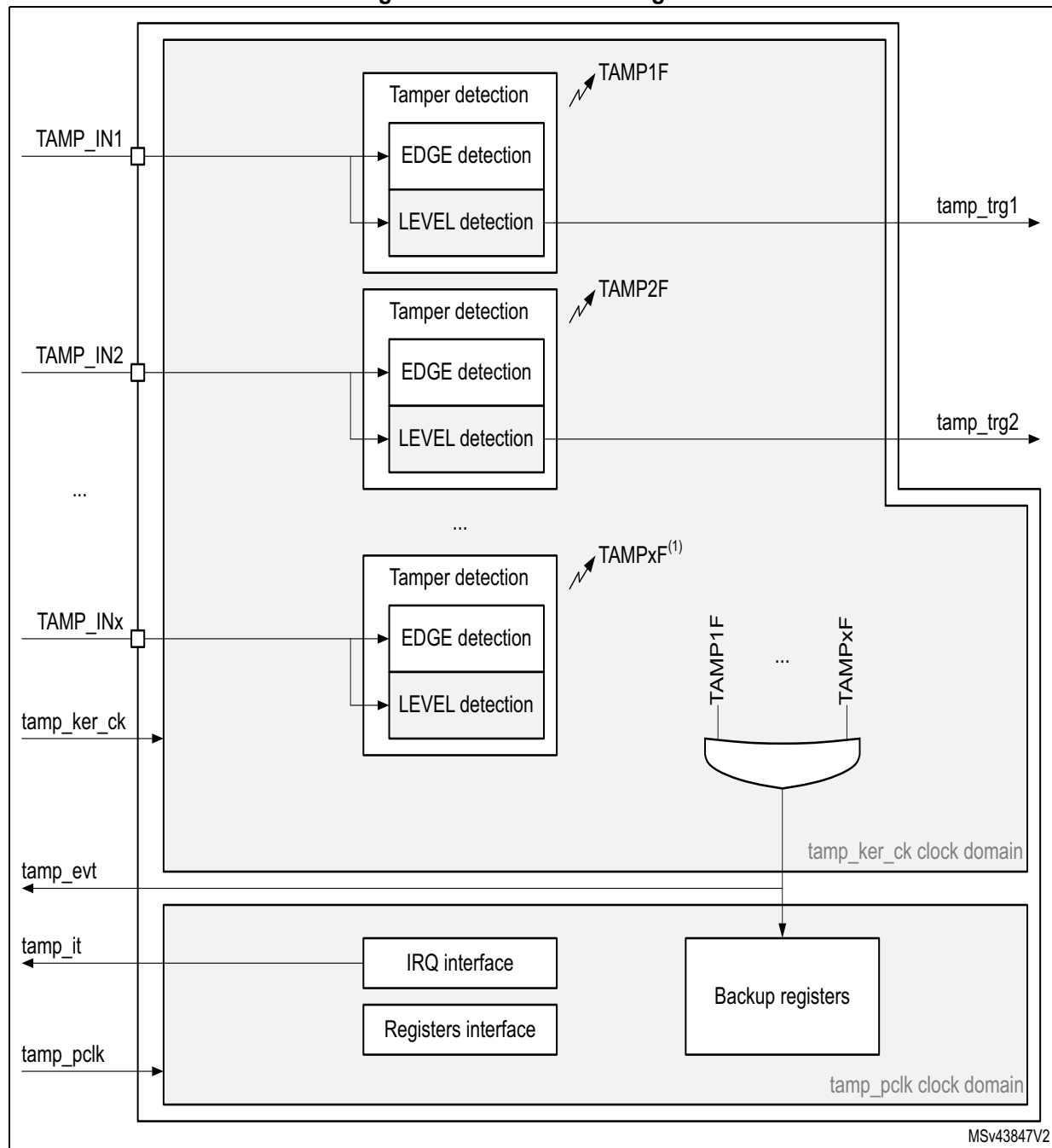
Figure 228. TAMP block diagram
