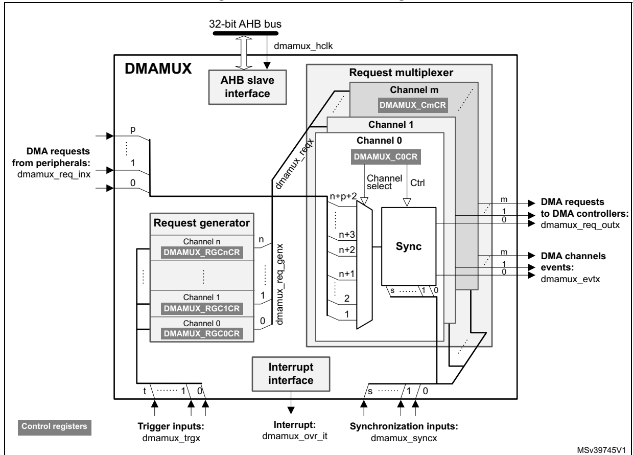
Figure 19. DMAMUX block diagram
