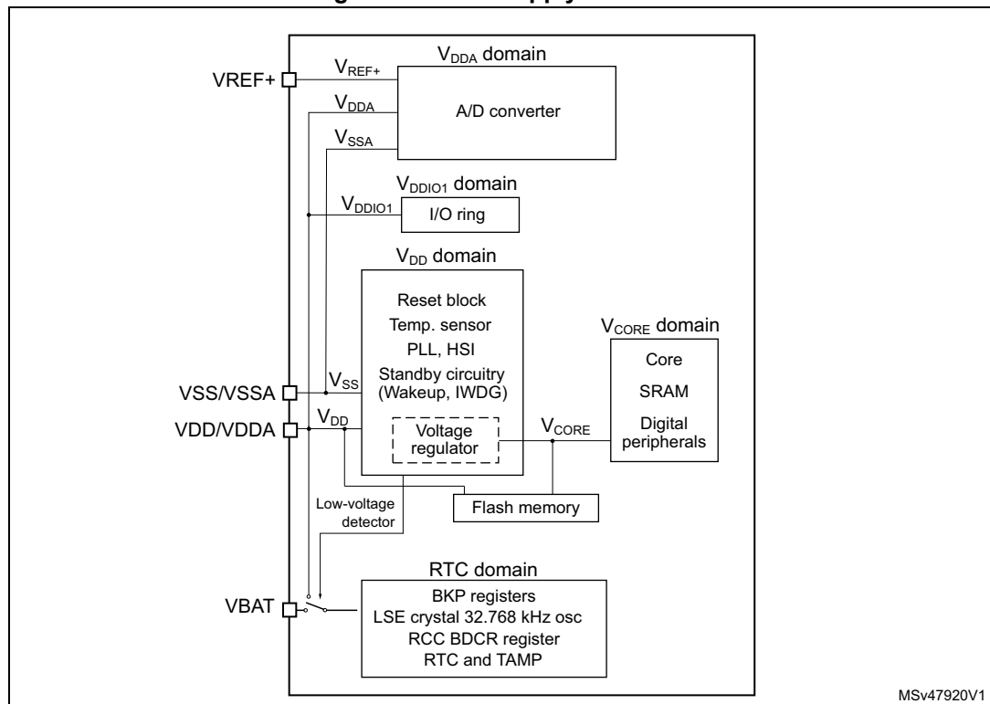
Figure 4. Power supply overview
