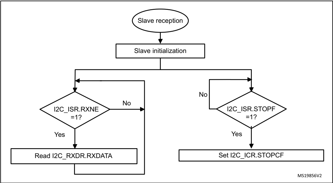
Figure 241. Transfer sequence flowchart for slave receiver with NOSTRETCH=1
