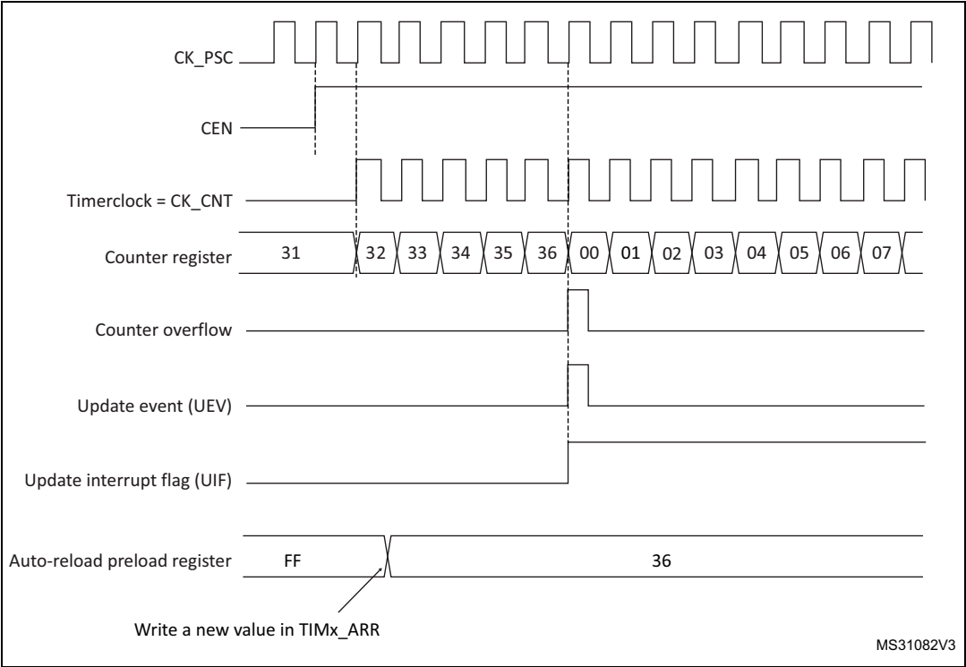
Figure 62. Counter timing diagram, update event when ARPE=0 (TIMx_ARR not preloaded)
