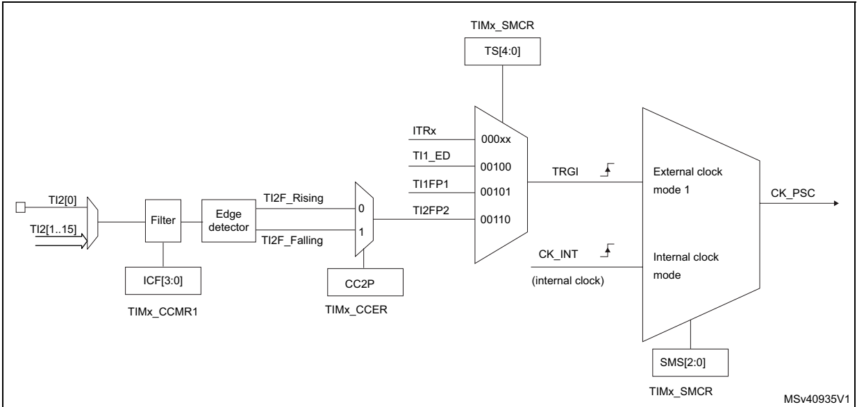
Figure 201. TI2 external clock connection example
