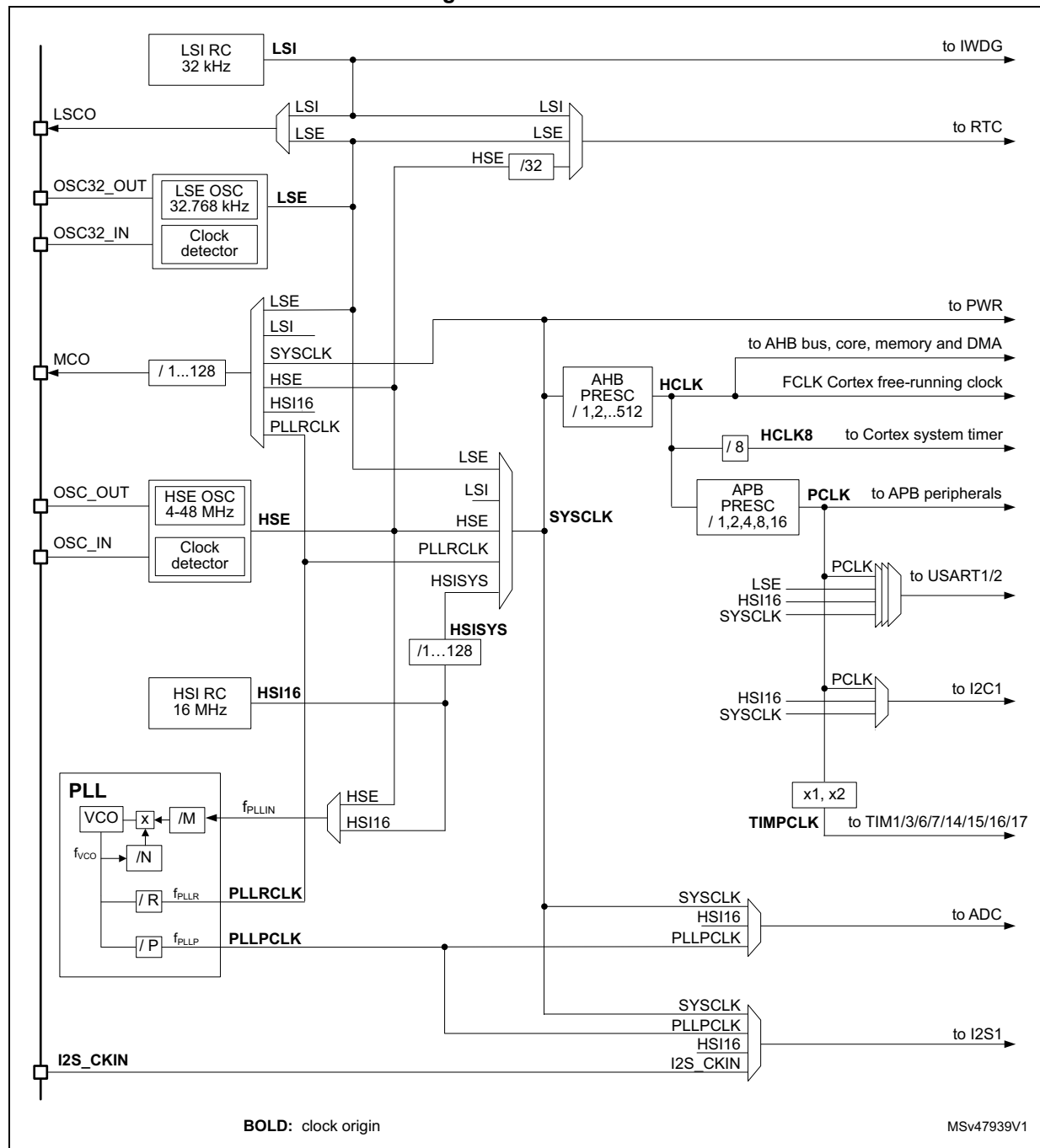
Figure 8. Clock tree
