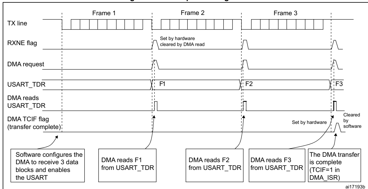
Figure 281. Reception using DMA
