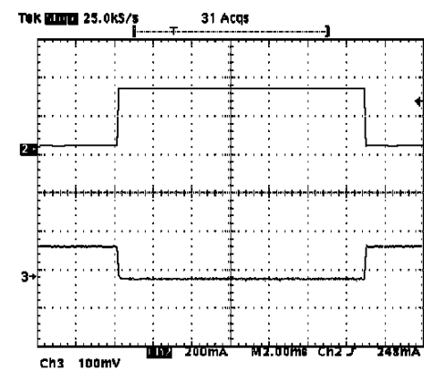
Figure 10 : Load Transient
