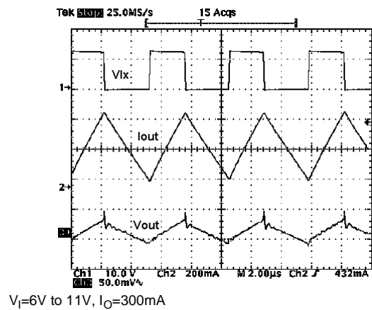
Figure 8 : Switching Waveforms, Discontinuous Conduction
